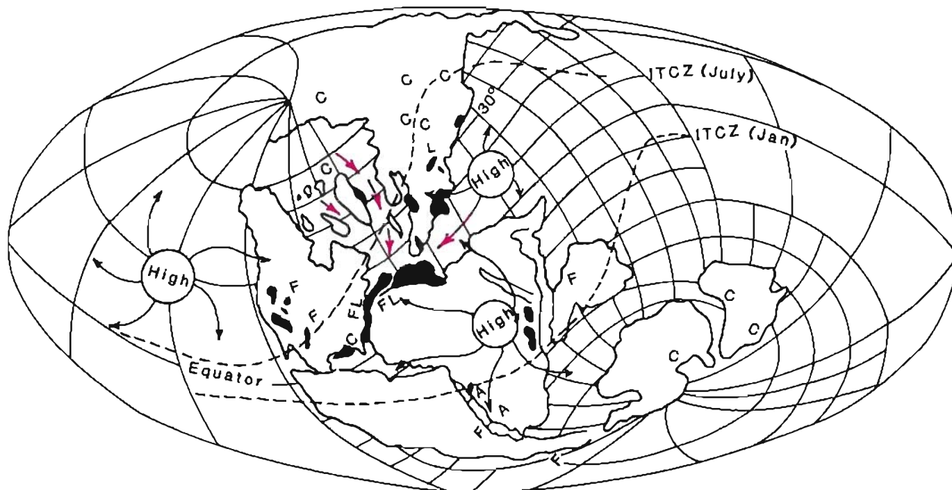
Figure 2. Position of the continents in the Late Triassic–Early Jurassic, showing the distribution of climate sensitive rocks, major high pressure cells and wind patterns for a Northern Hemisphere summer and Southern Hemisphere winter, and the location of the Intertropical Convergence Zone (ITCZ) for both seasons. The information, plotted on a Mollweide Projection, is modified from Robinson (1973). Evaporites are shown in black, A = aeolian sands, C = coal, F = fluvial strata, and L = lacustrine beds. Red arrows show two possible sources of Late Triassic marine transgression of the proto-Atlantic basins, one from the Tethys and the other from Arctic Canada (Manspeizer and Cousminer, 1988).
