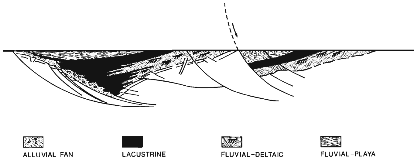
Figure 11. Geologic cross section of the Newark basin, drawn along the Delaware River, where the border fault is depicted as a listric normal fault merging with low-angle detachment faults that are inclined beneath the continental margin and where the distribution of major lithofacies is largely a function of the half-graben geometry. From Manspeizer, 1988.
