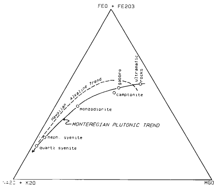
Figure 26. AFM ternary diagram showing the average Montegregian plutonic trend and the average Montegregian camptonite, compared with the Hawaiian alkaline trend.
